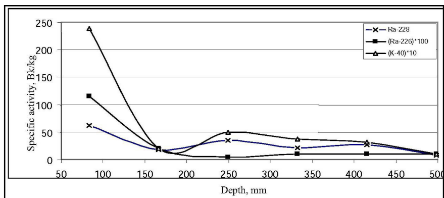
Figure 1. Distribution of natural radio-nuclide isotopes according to depth
