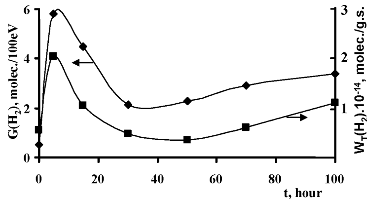
Fig.3. Dependences of radiation-chemical outlet and molecular hydrogen accumulation in ( \dot{D}=1.14\text{Gy/s} ) radiation-thermal (1) and thermal processes (2) of water decomposition at T=673\text{K} , \rho=5\text{mg/sm}^3 from the time of preliminary treatment of Zr, in contact with \text{H}_2\text{O}_2 at T=300\text{K} .
