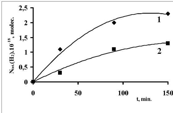
Fig.1. Kinetic curves of molecular hydrogen accumulation in radiation-thermal (1) ( \dot{D}=1.14\text{Gy/s} ) and thermal (2) processes of water decomposition in presence of Zr samples, previously radiationally treated at D=20,52 kGy in presence of \text{H}_2\text{O}_2 .
