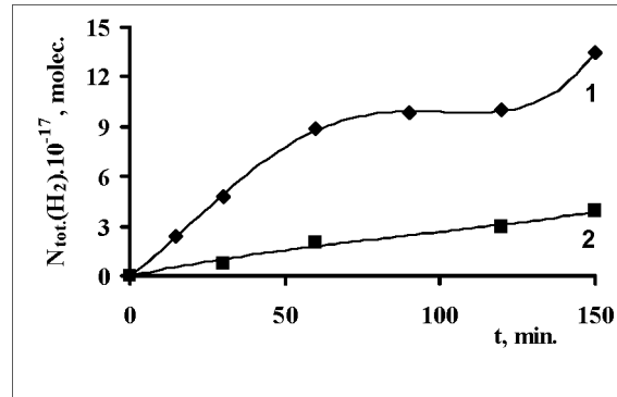
Fig.2. Kinetic curves of molecular hydrogen accumulation in radiation-thermal (1) ( \dot{D}=1.14\text{Gy/s} ) and thermal (2) processes of water decomposition in presence of Zr samples, previously radiationally treated at D=287,28 kGy in presence of \text{H}_2\text{O}_2 .
