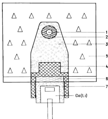
Fig.1. Schematic graph of the device
