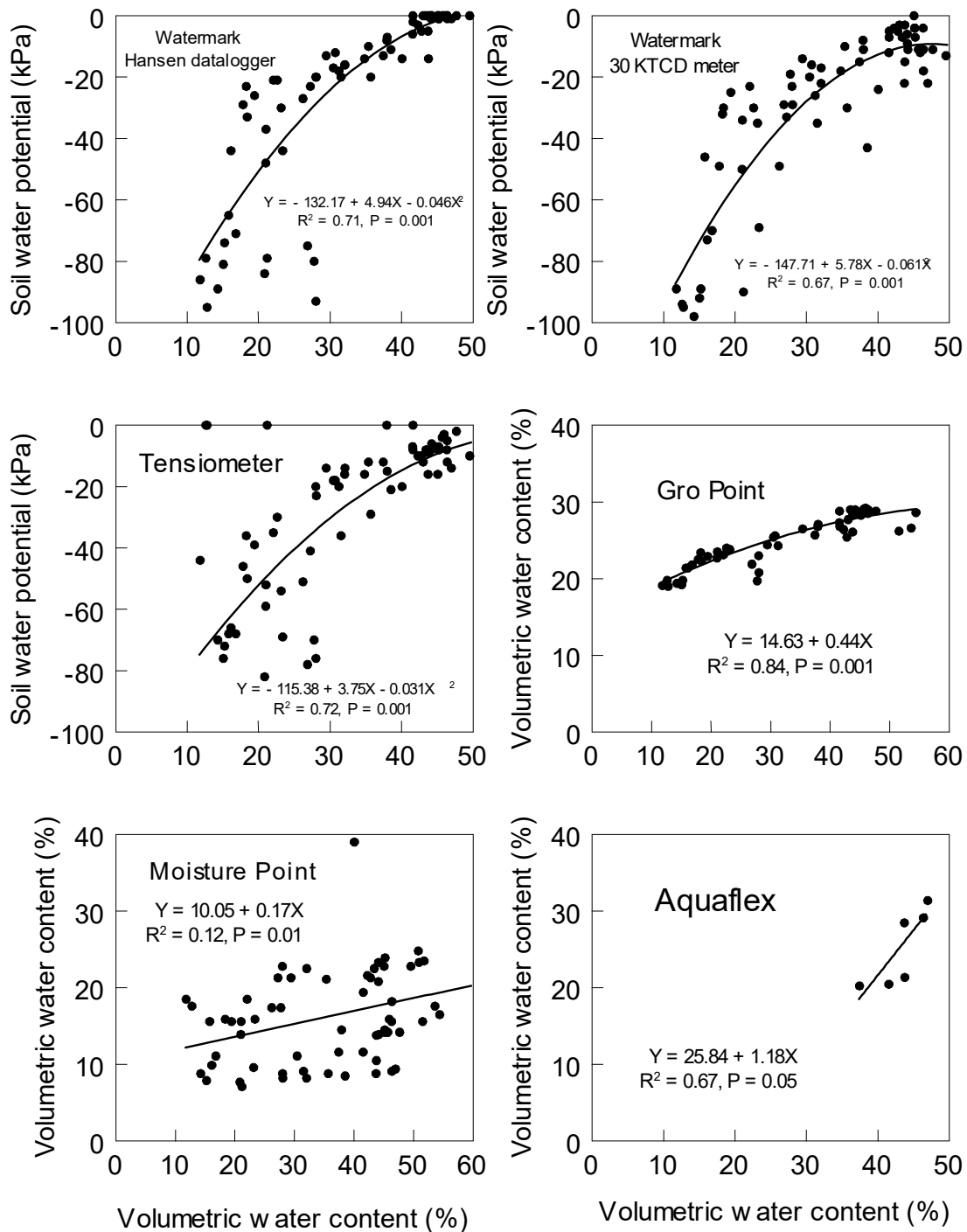
Figure 6. Volumetric soil water content measured in Experiment 2 by a neutron probe (X axis) regressed against soil moisture data (Y axis) measured by 6 types of soil moisture sensor.
